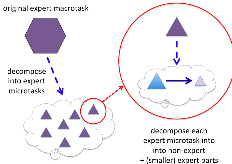
Fig. 4. Decomposing microtasks.
